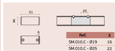
SM.010C - Ø19 SM.010C - Ø25 Conector para tubo / Tube conector / Conector de tubo.
